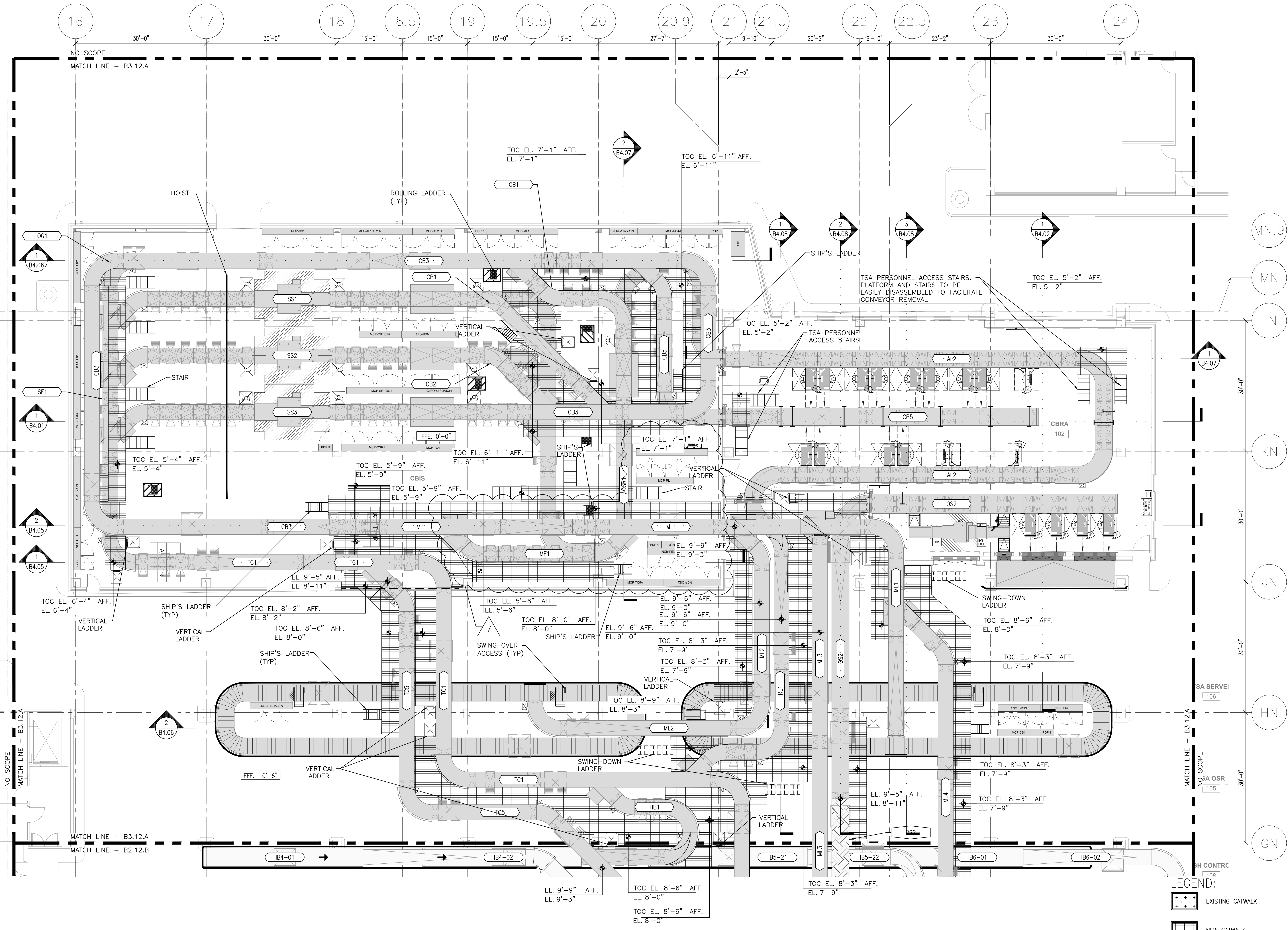
1 PARTIAL PLAN - BAGGAGE LEVEL - PROPOSED CATWALK - ZONE A - NORTH BAGROOM - 1/8"=1'-0" SCALE
